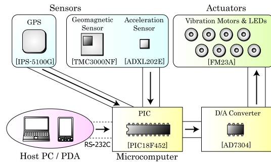
図3 Active Belt システム構成 Fig. 3 System architecture of Active Belt
