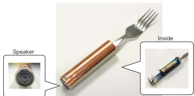
Figure 2: The prototype of Analog EaTheremin.
