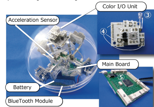
figure 2. Device architecture of ChameleonBall: (1) color sensor (TAOS TCS230), (2) infrared reflection sensor (Sharp GP2S40), (3) white LED, (4) full-color LEDs (Osram LATBT66B), and (5) microcomputer (Microchip PIC18F2550)
