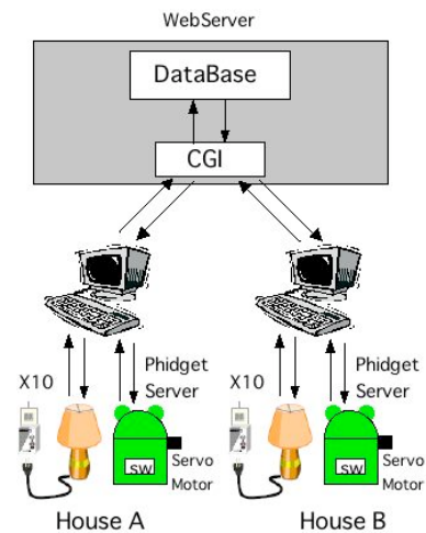
figure 3. Overview of the SyncLamp and SyncTrash systems
